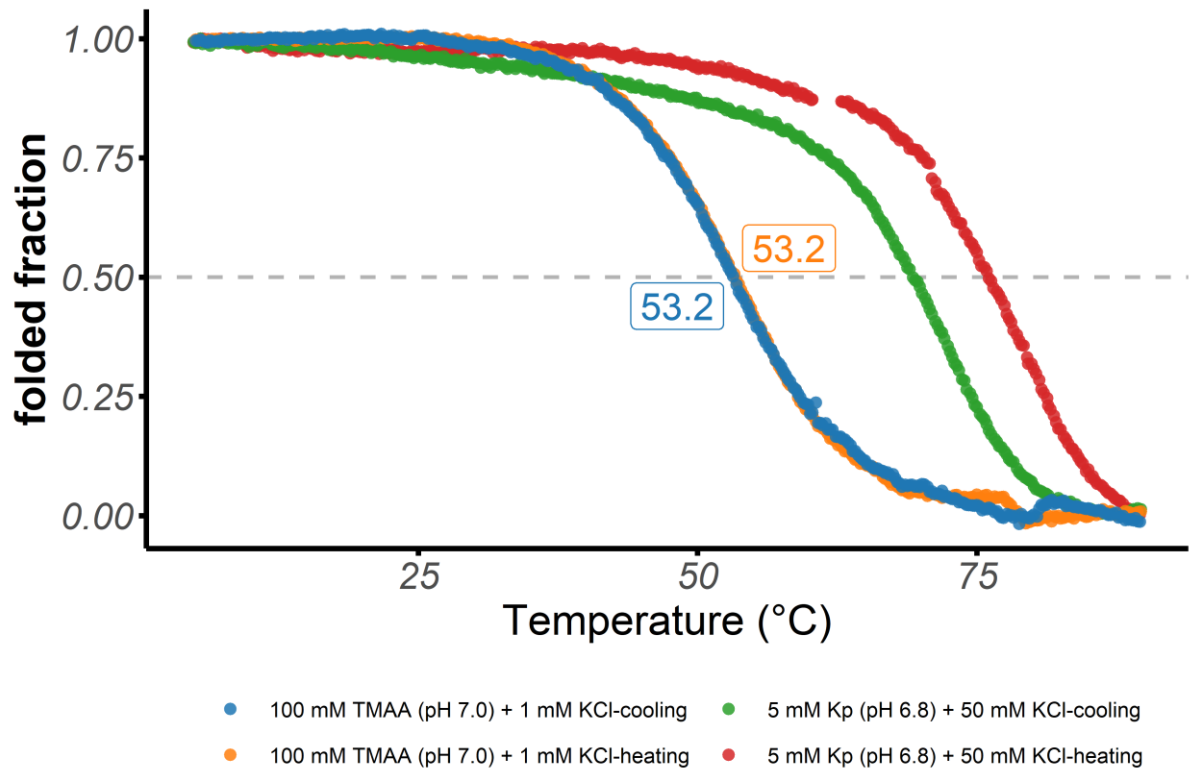
Folded fraction of the 2KPR oligonucleotide as a function of temperature, determined by UV-melting ( \lambda = 295 \text{ nm} )
