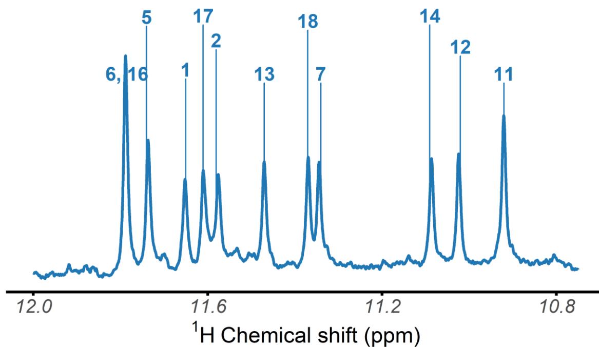
^1\text{H} -NMR spectrum of the 2KPR oligonucleotide, acquired at 25°C in 100 mM TMAA (pH 7.0) + 1 mM KCl
